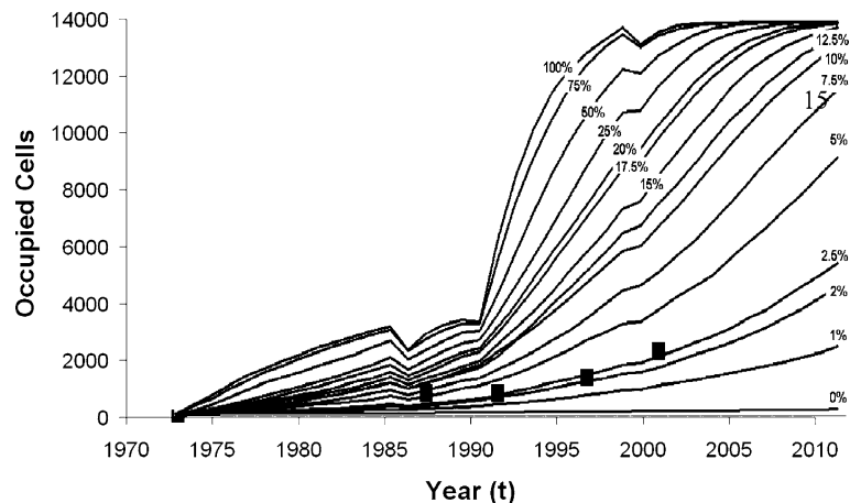
Fig. 3 Effect of long-distance dispersal on invasion in exemplary simulation runs in the standard landscape scenario. The categories of long-distance dispersal are based on the percentage of the total number of offspring involved in long-distance dispersal events. The changes in
