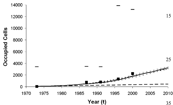
Fig. 4 Number of all occupied grid cells ( 5 \times 5 m) in the simulation model of Heracleum mantegazzianum (line with SD). Land-use changes occurred in the years t = 1987, 1991, 1996, and 2000 . Horizontal lines indicate the maximum number of grid cells that can be occupied at those times (except for scenario 3 where max. number remains constant at the level of 1973). Observed spread (squares) lies slightly above the values for the standard scenario (scenario 1, full line). The populations without long-distance dispersal (scenario 2, long broken line) only exhibit moderate increase. Populations in non-changing landscapes are showing the same increase in number of occupied cells as those in a shifting scenario (scenario 3, short broken line). Detailed values for the historical data are presented in Table 2
