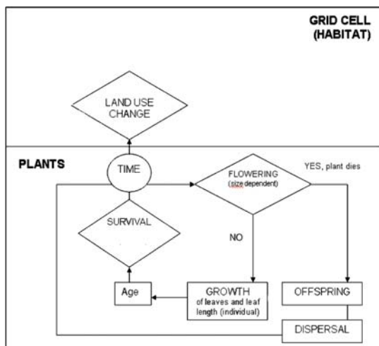
Fig. 1 Flow chart of the individual-based model of Heracleum mantegazzianum . Within one time-step (year) different probabilities determine the fate of an individual plant. Changes in landscape structure (i.e., if one land-use type changed into another) were incorporated in the model in the year when observed on aerial photographs. Rhombs represent decisions, boxes are mandatory developments
