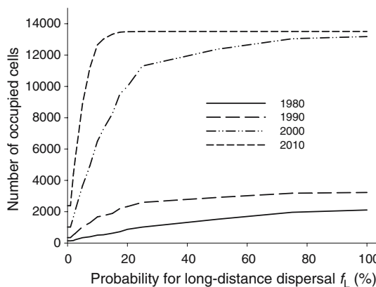
Fig. 5 Number of occupied cells for 1980, 1990, 2000, and 2010 in relation to the implemented probability for long-distance dispersal ( f_L ). Lower probabilities have over-proportionally higher effect on cell occupation than high probabilities
